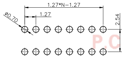
RECOMMEND PCB LAYOUT (TOLERANCE=±0.05)
