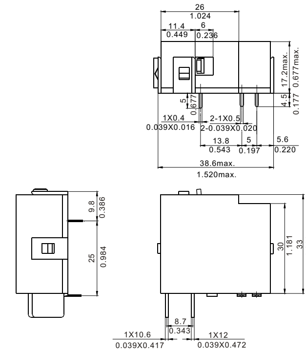
Dimensions Mounting (Bottom view)
