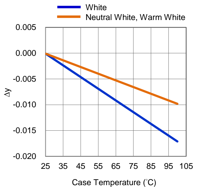
Fig 4. Case Temperature vs. Chromaticity Coordinate \Delta y at 540mA.
