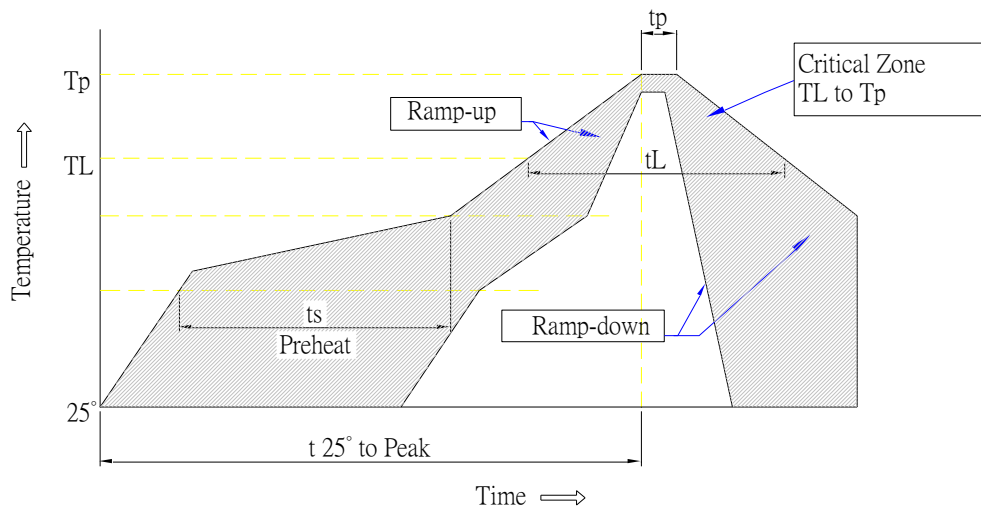
Temperatures profile
