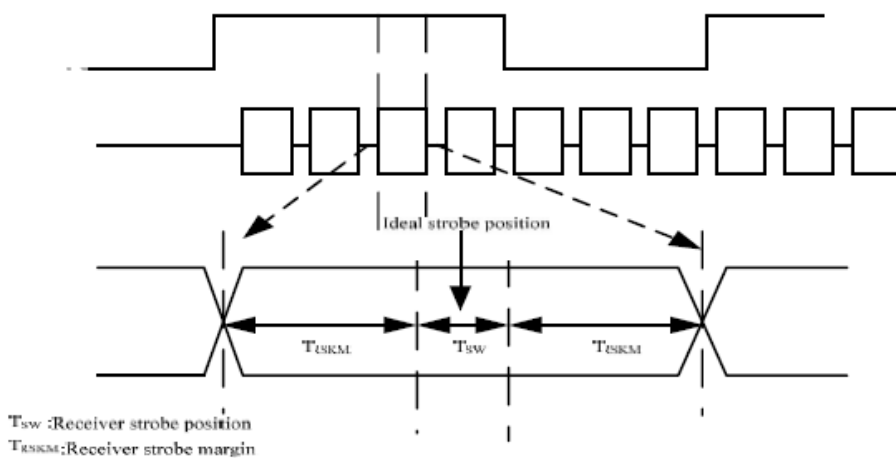
LVDS timing(3)
