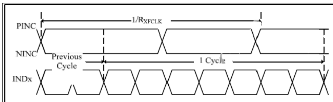
LVDS timing(1)
