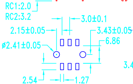
PCB Layout: Component side
