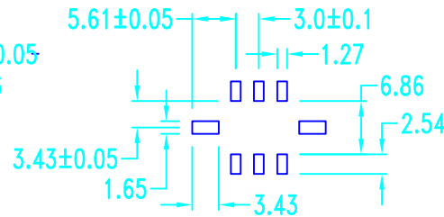
PCB Layout: Component side
