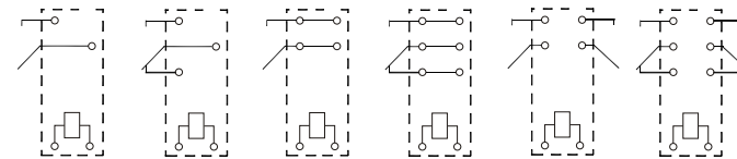
Wiring diagram (Bottom view)
