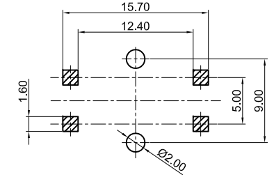
RECOMMEND PCB LAYOUT(Tolerance=±0.05)
