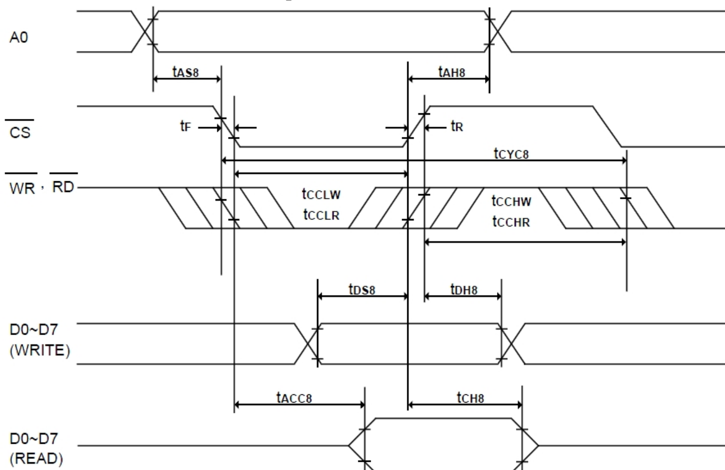
8080-series parallel interface characteristics
