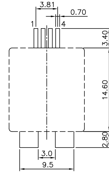
RECOMMENDED PCB LAYOUT AS VIEWED FROM COMPONENT SIDE
