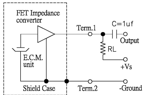
Schematic Diagram
