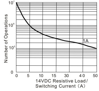
Endurance Cruve
