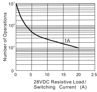
Endurance Cruve
