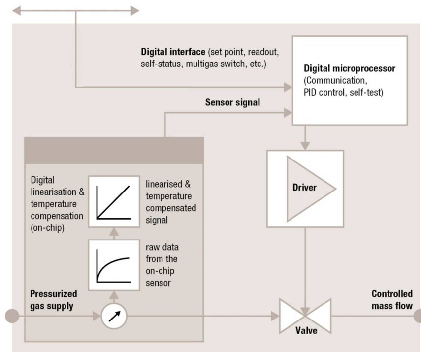
Figure 2: Block diagram CMOSens® SFC5500 mass flow controller.
