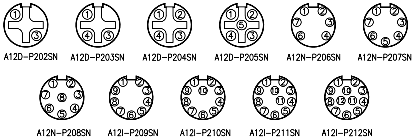
Pin Assignment Front View (前視圖)
