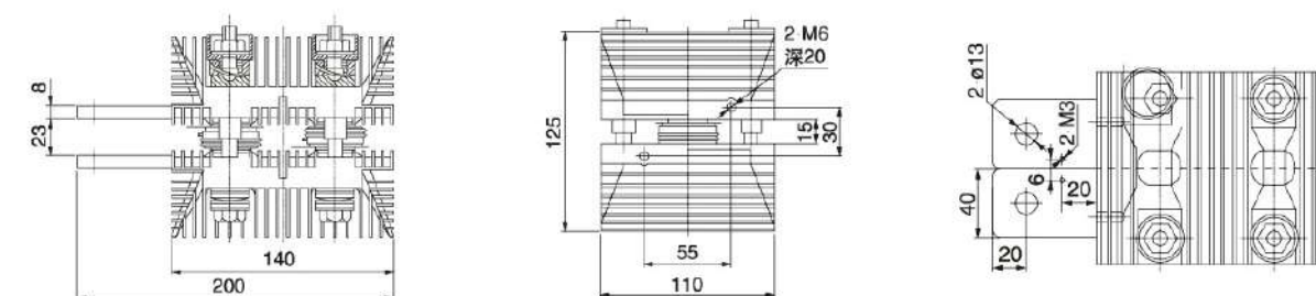
SF15BL Double Devices Air-cool Heatsink
