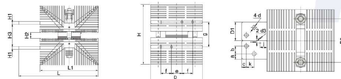
SF14, SF15, SF16, SF17 Air-cool heatsink
