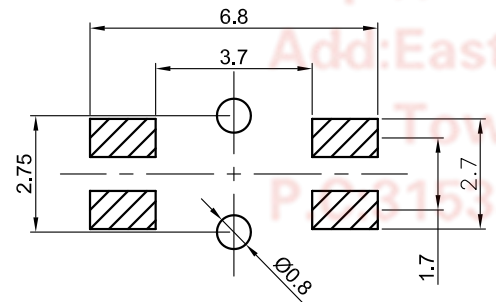
PCB hole layout Tolerance±0.05
