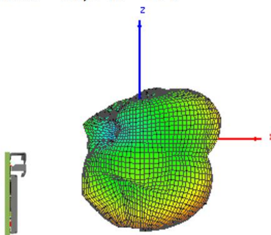
Theta = 90, Phi = 270
