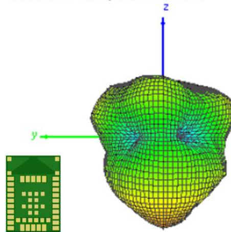
Theta = 90, Phi = 180
