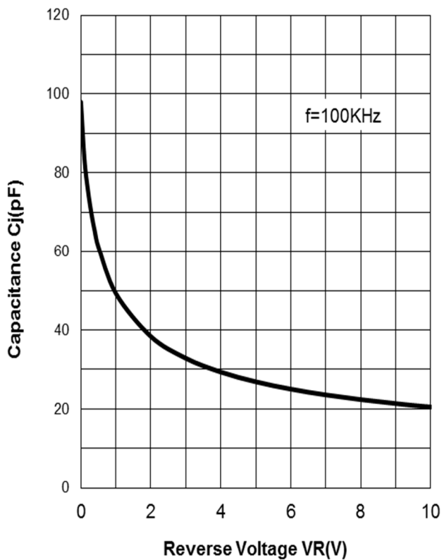
Capacitance vs. Reverse Voltage (Ta=25°C)
