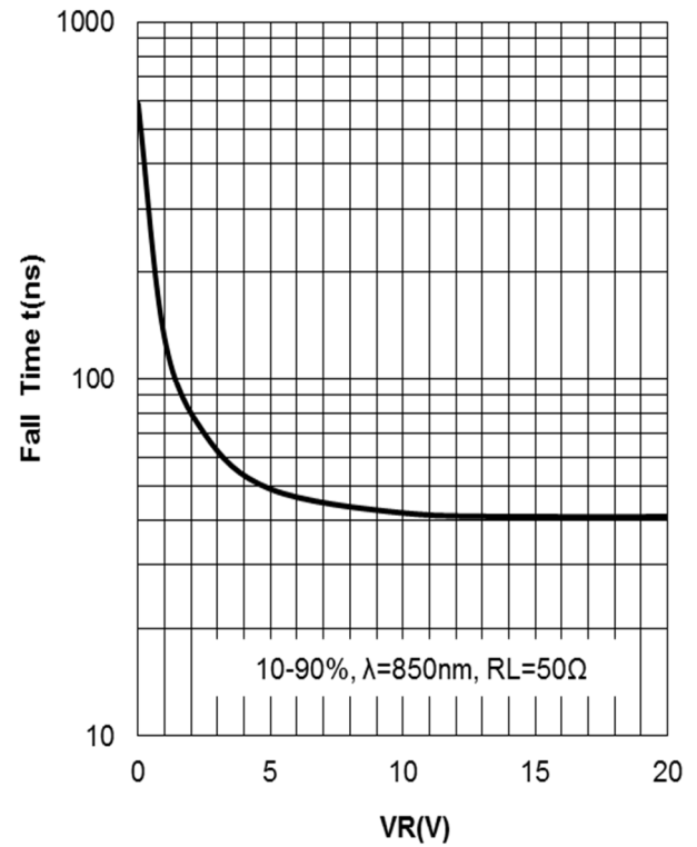
Fall Time vs. Reverse Voltage (Ta=25°C)
