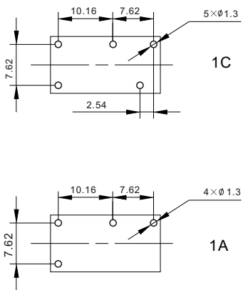
Mounting (Bottom view)
