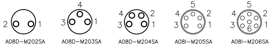
PIN ASSIGNMENT FRONT VIEW (前視圖)
