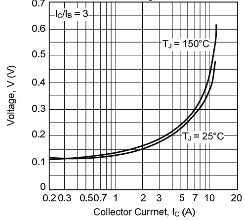
Fig. 8 Collector - Emitter Saturation Voltage
