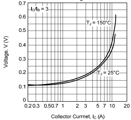
Fig. 8 Collector - Emitter Saturation Voltage
