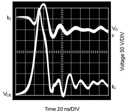
Fig. 13 Typical Inductive Switching Waveforms (at 300V and 12A with I B1 = 2.4A and V BE(off) = 5V)
