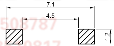
PCB Layout Tolerance±0.05
