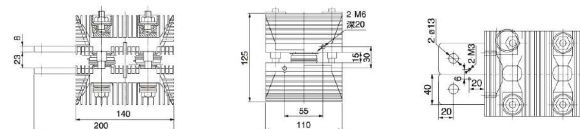
SF15CL Double Devices Air-cool Heatsink
