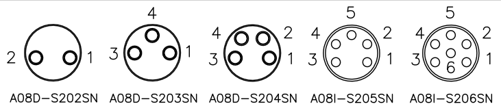
PIN ASSIGNMENT FRONT VIEW (前視圖)
