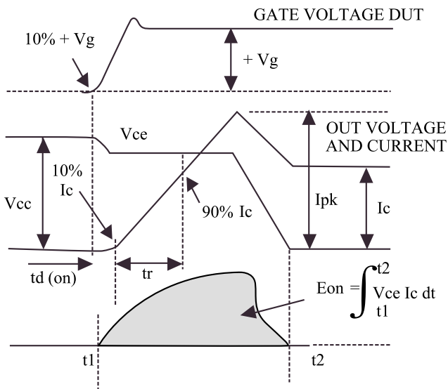
Fig 21. Definition Switching Time & Loss
