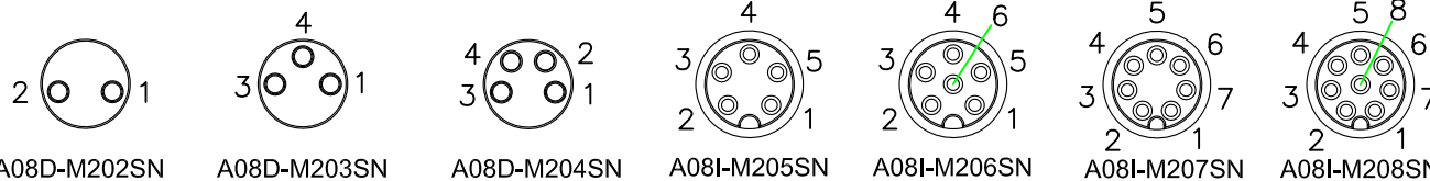
PIN ASSIGNMENT FRONT VIEW (前視圖)
