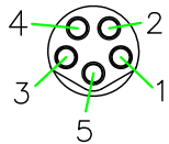
PIN ASSIGNMENT FRONT VIEW
